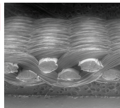
Flowrox W-TA220L filter cloth, electron microscope image.
