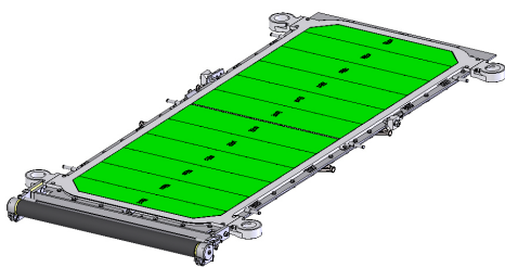
Flowrox 6 m 2 complete filter plate
