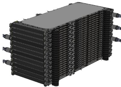
Flowrox plate pack TP 144 60 1 60
